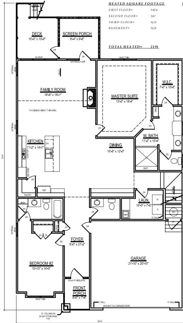
FIRST FLOOR PLAN CEILING HT. = 9'-0"
