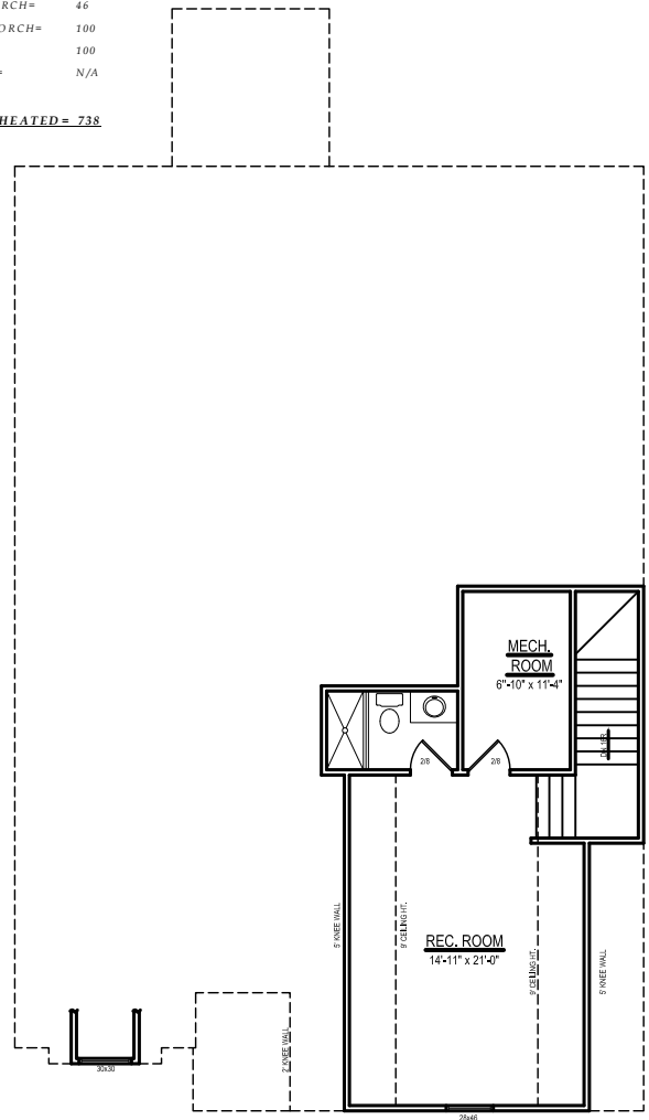
SECOND FLOOR PLAN CEILING HT. = 9'-0"
