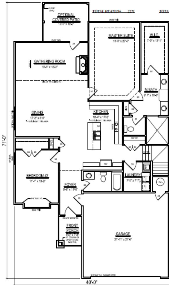
FIRST FLOOR PLAN CEILING HT. 8'-0"
