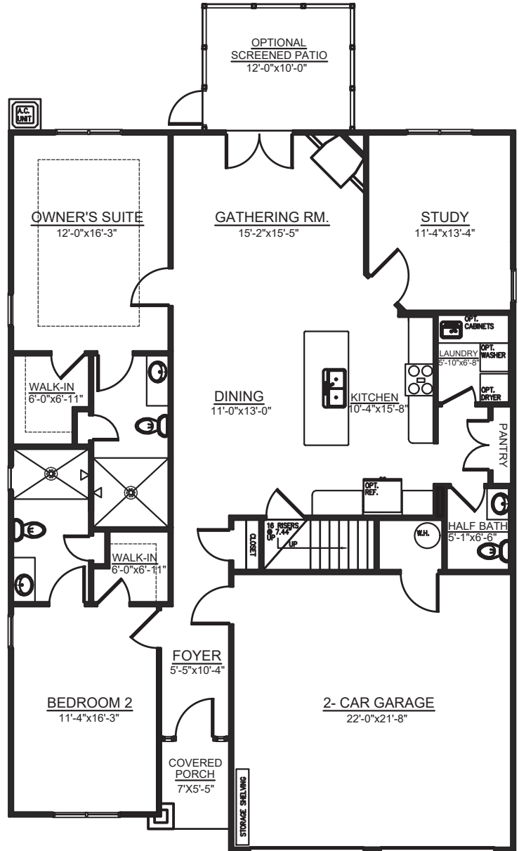
1 FIRST FLOOR PLAN A101 | SCALE: 3/32"=1'-0"
