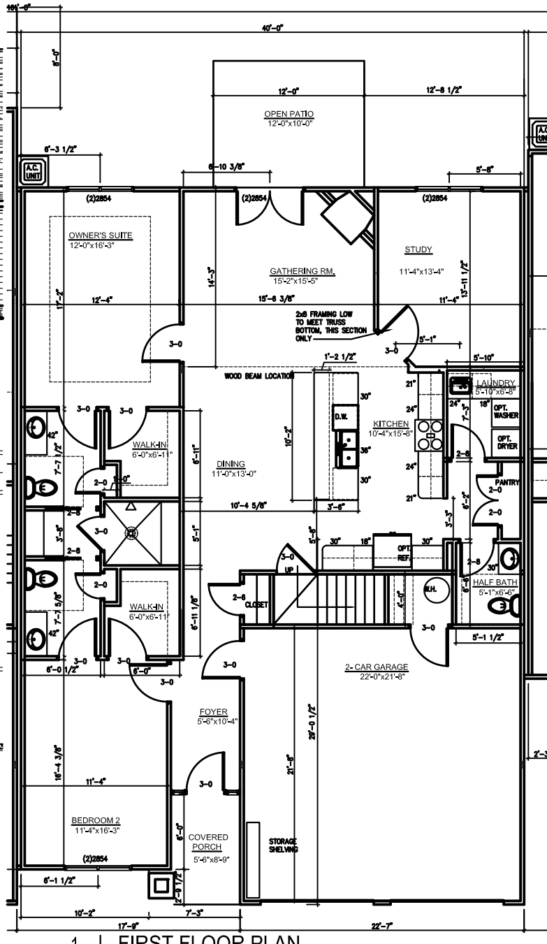
1 FIRST FLOOR PLAN
